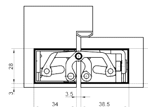
Cross section for TE 526 3D with intumescent kit Ref. 8820
